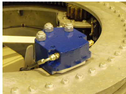
CLAVIJO'S AZIMUTHAL BRAKE SYSTEM
